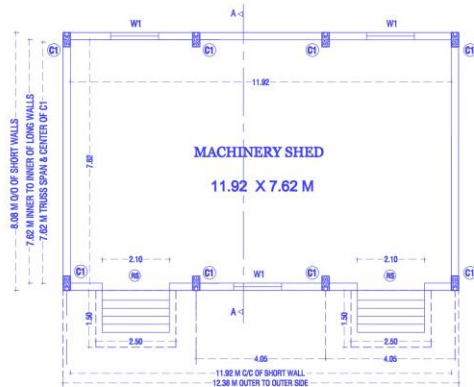
MACHINERY SHED PLAN
